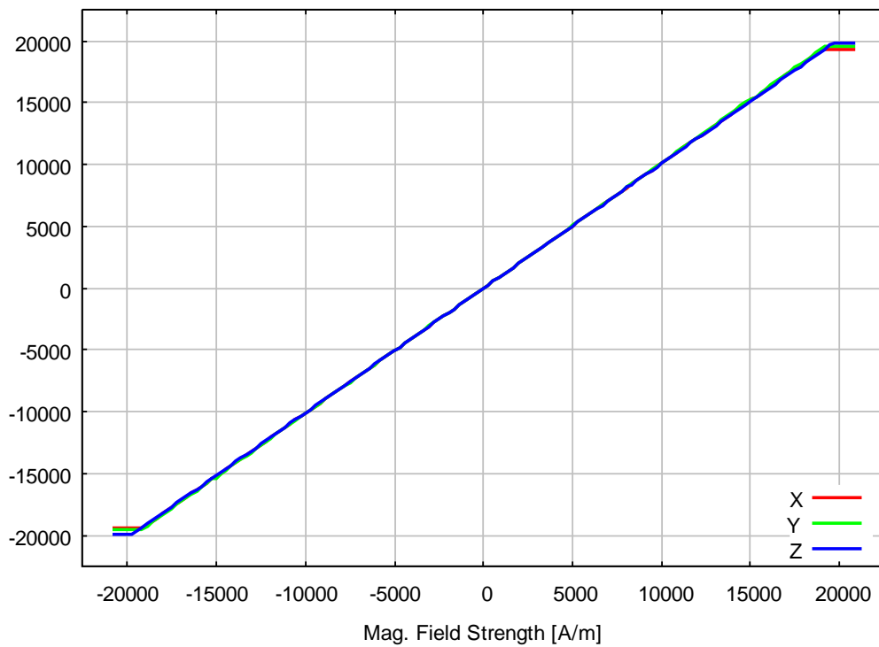
Linearity, measuring range 20000A/m
