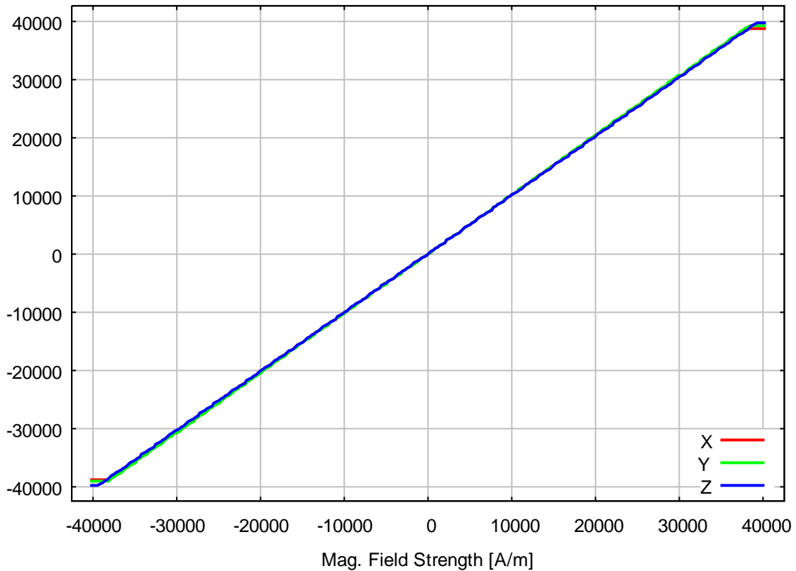
Linearity, measuring range 40000A/m
